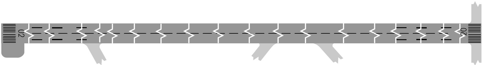
MARKING AIDS RWY 02 / 20 AND EXIT TWY
