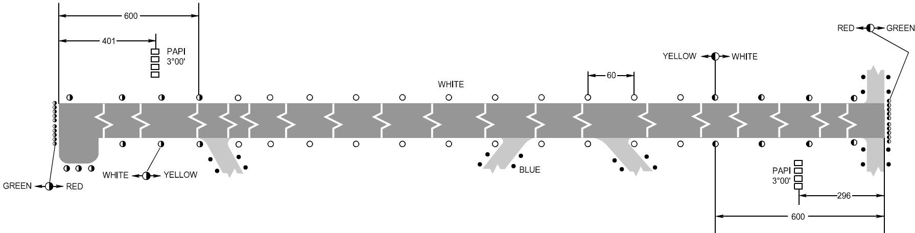
LIGHTING AIDS RWY 02 / 20 AND EXIT TWY
