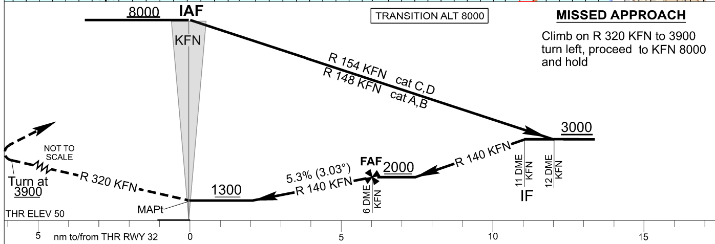
Altitude (Height) on Final Approach
